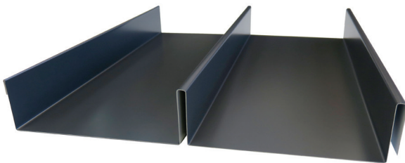
Oceania
